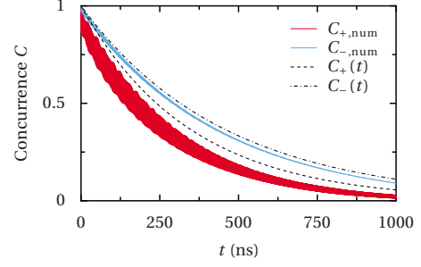
FIG. 7. (Color online) Decay of concurrence C_+ and C_- for the entangled initial states |\psi_+\rangle_{\text{cav}} and |\psi_-\rangle_{\text{cav}} (solid red lines, thick curve, and solid blue lines, thin curve, respectively). The switch-setting off condition g_{\text{SW}}=0 is fulfilled by \varepsilon/2\pi = -8.916 \text{ GHz}/2\pi . Here we use G=0.00478 \text{ GHz} , all other parameters are as in Fig. 3. The exponential decay corresponds to Eqs. (44) and (45) (black dashed and dash-dotted lines, respectively).
